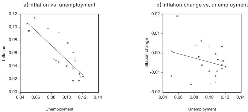
Figure 2: Covariation in Inflation and Unemployment
