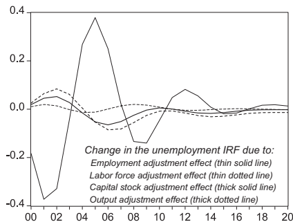
Figure 6: The Influence of Real Rigidities (Persistence is Reduced by 10% in Each Real Equation)
