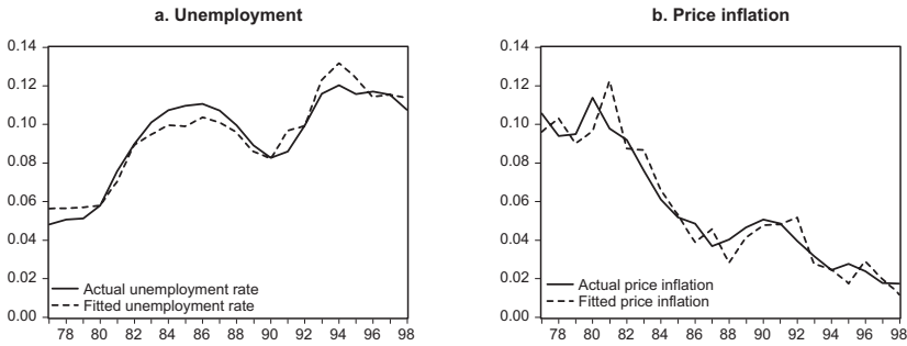
Figure 4: EU Unemployment and Price Inflation: Actual and Fitted Values
